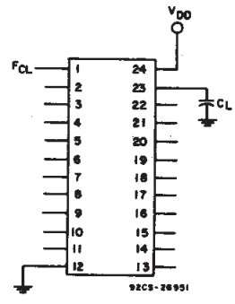
Fig. 19 - Power dissipation test circuit (all \div modes).
