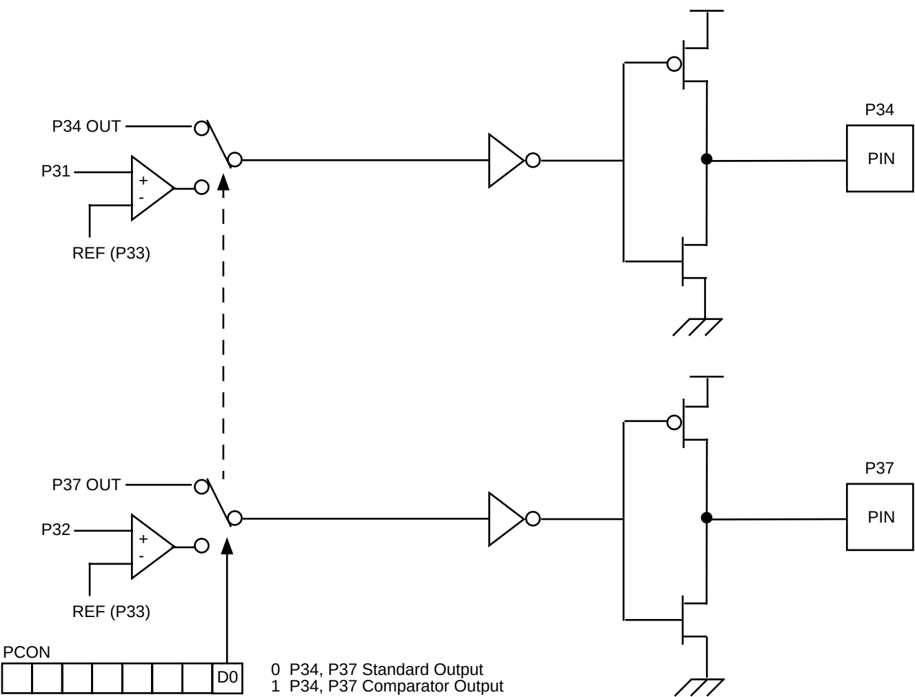
Figure 5-33. Port 3 Configuration
