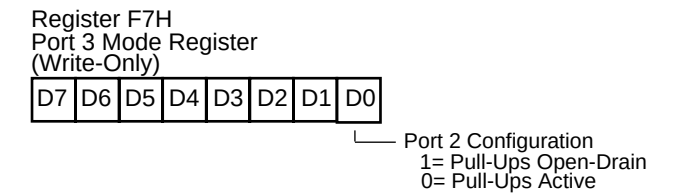
Figure 5-34. Port 2 Configuration
