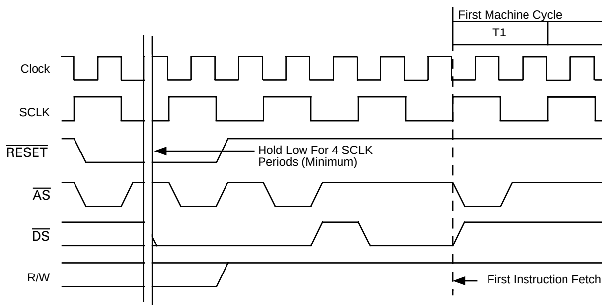
Figure 4-1. Reset Timing
