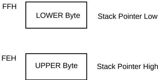
Figure 2-9. Stack Pointer
