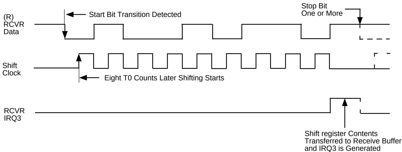
Figure 9-6. Receiver Timing
