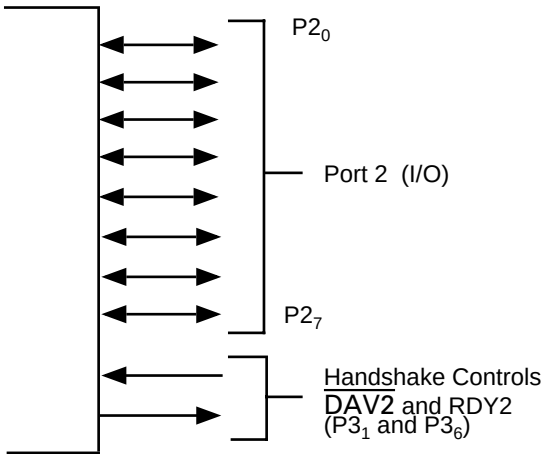
Figure 5-16. Port 2 Handshaking
