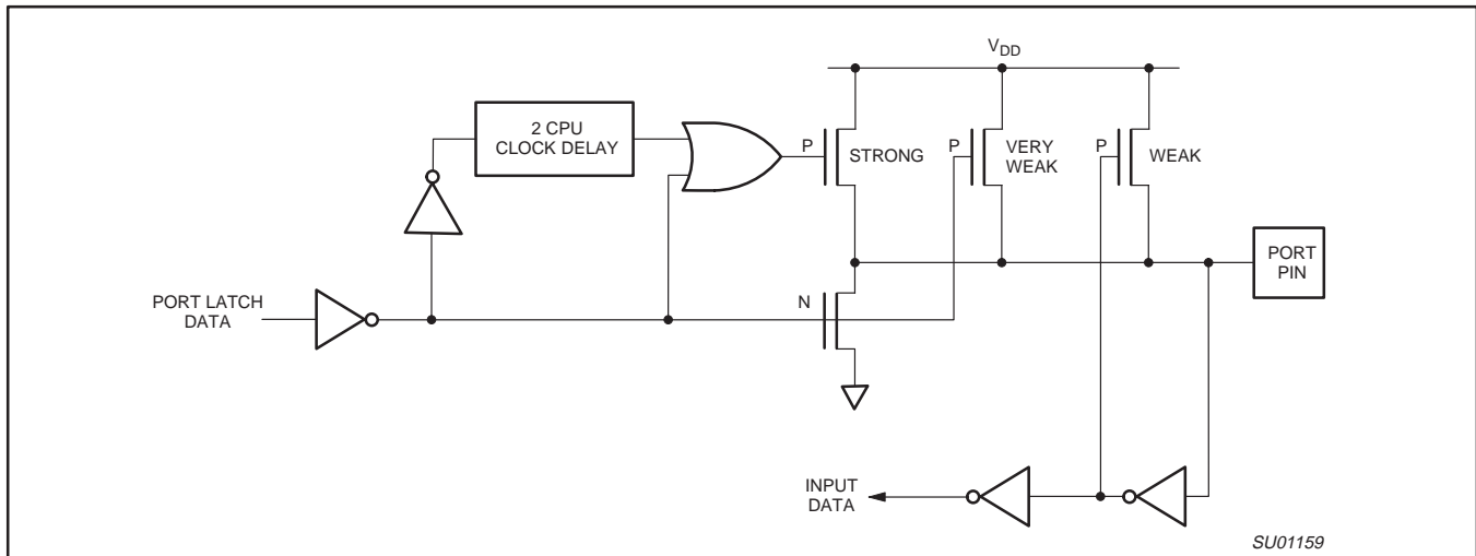
Figure 12. Quasi-Bidirectional Output
