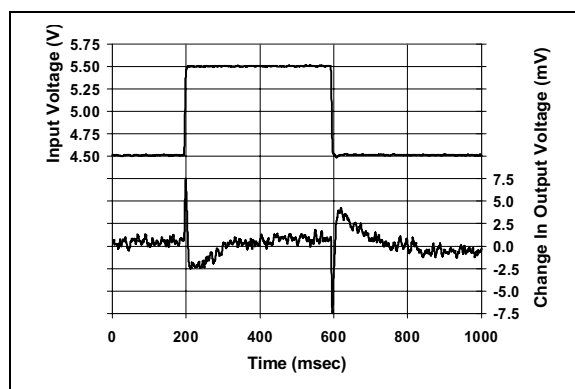
FIGURE 2-17: MCP1525 Line Transient Response.
