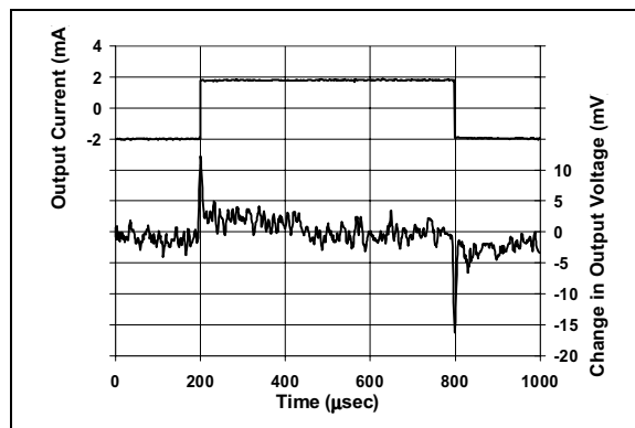
FIGURE 2-16: MCP1525 Load Transient Response.
