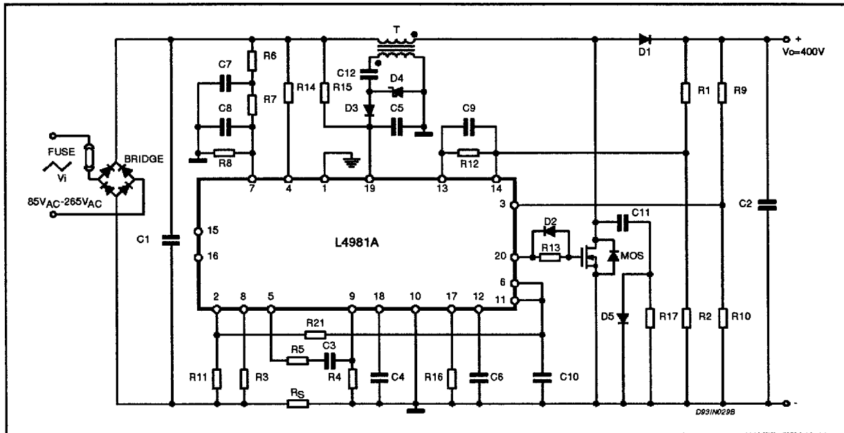
Figure 9A: L4981A Power Factor Corrector (200W)
