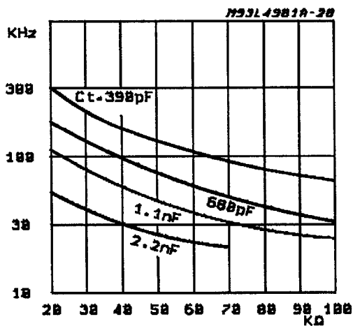
Figure 18: Oscillator Diagram
