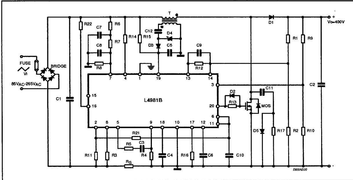
Figure 9B: L4981B Power Factor Corrector (200W)
