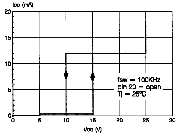
Figure 15: Operating Supply Current vs. Supply Voltage
