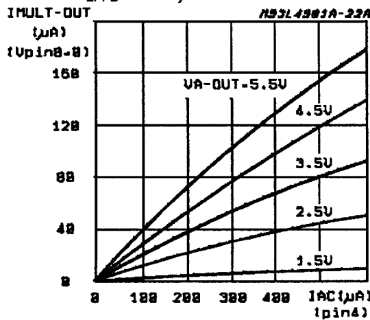
Figure 7: MULTI-OUT vs. I AC (V RMS = 4.4V; V LFFD = 2.5V)
