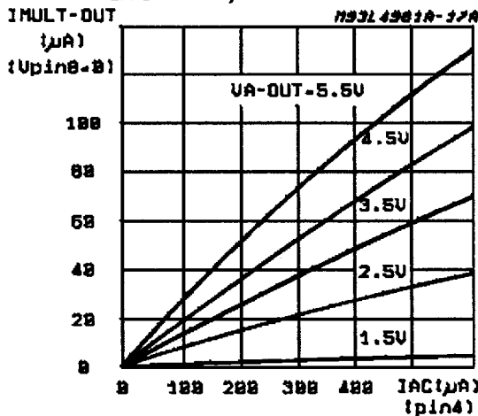
Figure 3: MULTI-OUT vs. I AC (V RMS = 4.4V; V LFFD = 5.1V)
