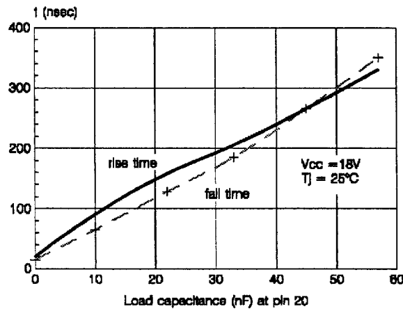
Figure 14: Gate Driver Rise and Fall Time
