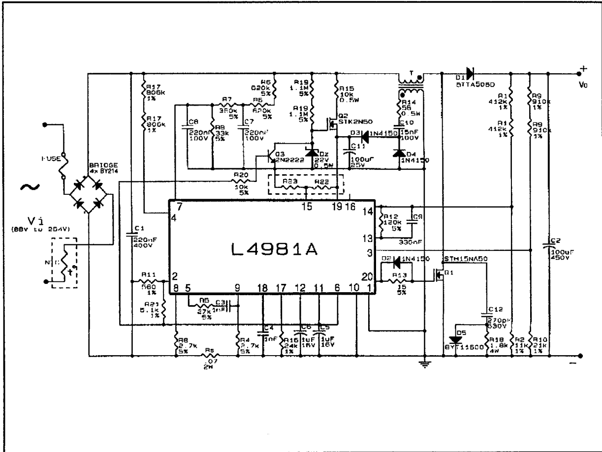
Figure 19: 200W Evaluation Board Circuit.
