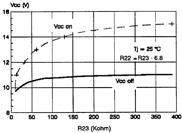
Figure 16: Programmable Under Voltage Lock-out Thresholds
