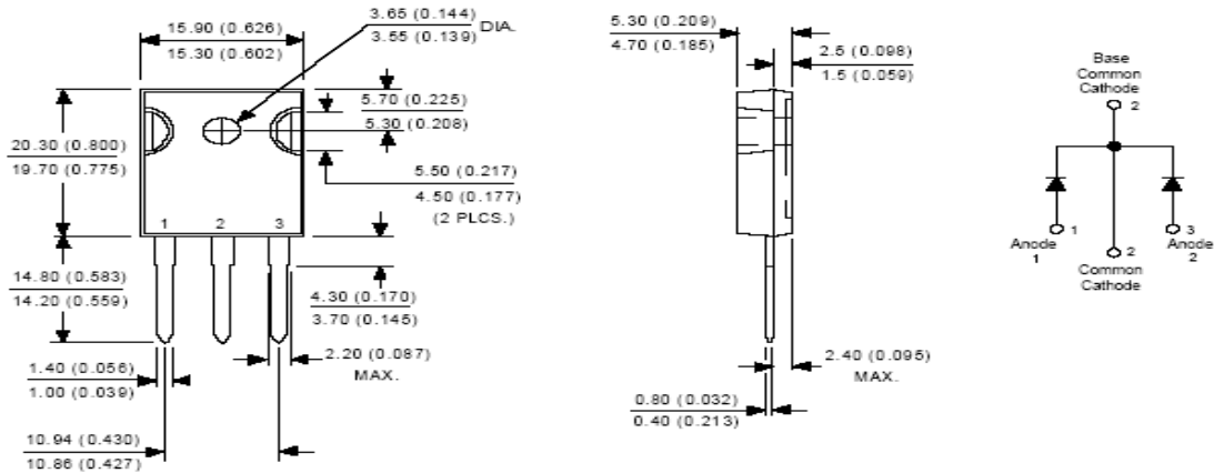
Conform to JEDEC outline TO-247AC (TO-3P) Dimensions in millimeters and (inches)
