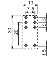
41.61 41.81 - 8240 95.15.2 Copper side view
